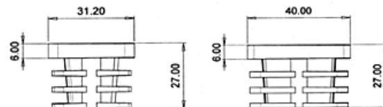
SQUARE RIBBED INSERT 30x30 - 40x40 material polyethylene
