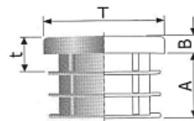
OVAL RIBBED INSERT material polyethylene
