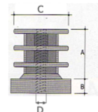
THREADED SQUARE RIBBED INSERT 25x25 - M8-M10 material polyethylene
