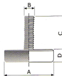
ADJUSTABLE FEET WITH OR WITHOUT HEXAGONAL HEAD
