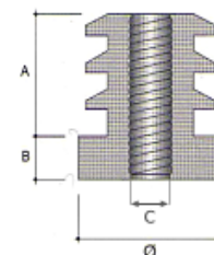
THREADED ROUND RIBBED INSERT M8-M10 material polyethylene
