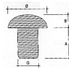
ROUND HEAD BUFFER \varnothing 24 mm material polyethylene
